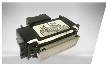
RICOH GH2220 Printhead 3.5PLink drop
